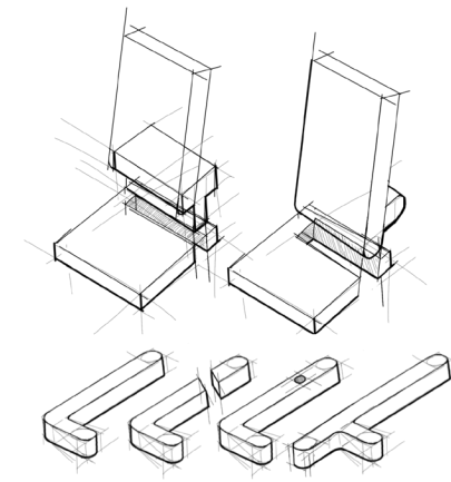
CNC MANUFACTURING, GLUE-UP ASSEMBLY OF PLYWOOD PIECES
